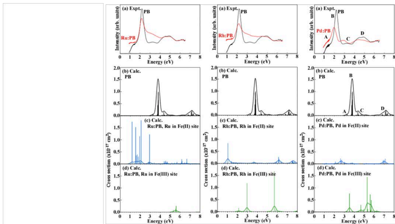
Figure 27. Theoretical spectra of the pristine (b) and PGMs-sorbed PB using the cluster models for \text{Fe}^{2+} (c) and \text{Fe}^{3+} (d) substitution, along with the experimental UV-vis-NIR spectra of PB before (black) and after (red) PGMs sorption (a).
