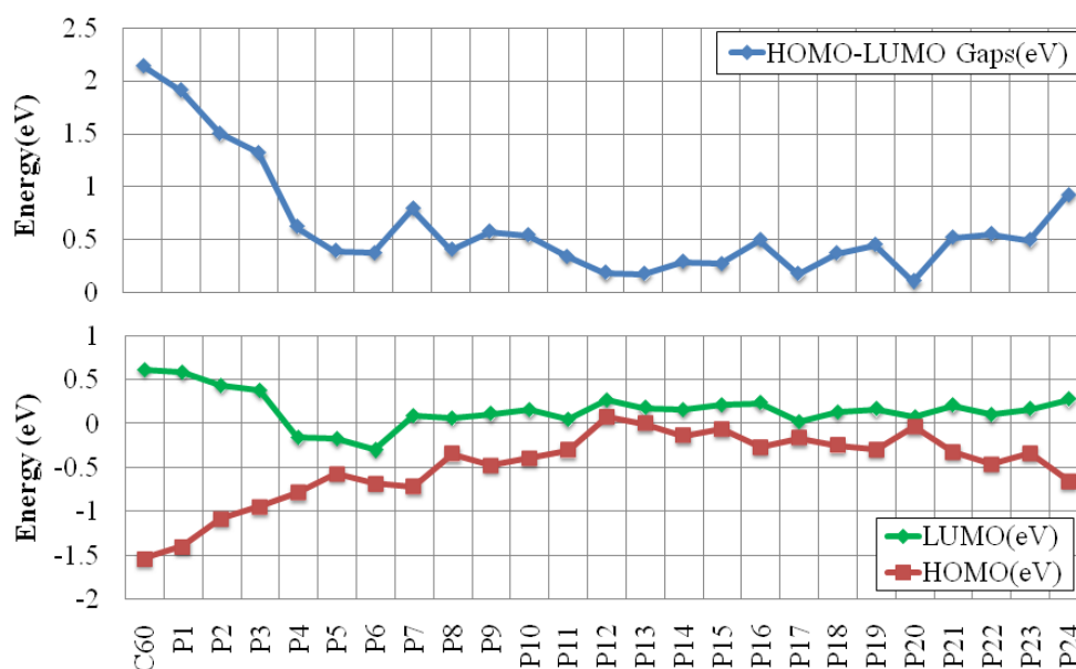
Figure 19. The HOMO-LUMO gap (top) and the energy level of the HOMO and LUMO (bottom) for each C_{120} isomer [28].
