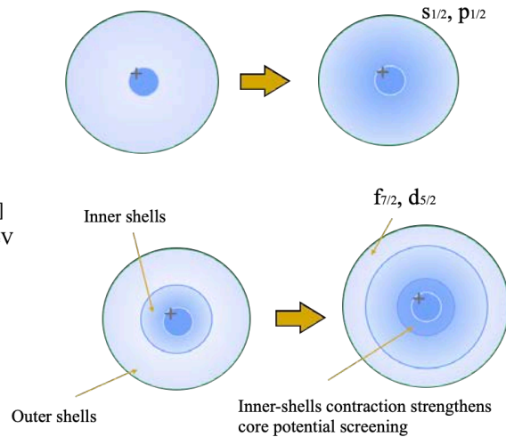
Figure 1. Schematic illustration of relativistic effects on atomic orbitals: (1) Direct effects such as the contraction of inner-shell AOs (s and p orbitals) and spin-orbit coupling (for an example, 6p AO splits to 6p 1/2 and 6p 3/2 AOs), (2) Indirect effect such as expansion of outer-shell AOs (d and f orbitals).
