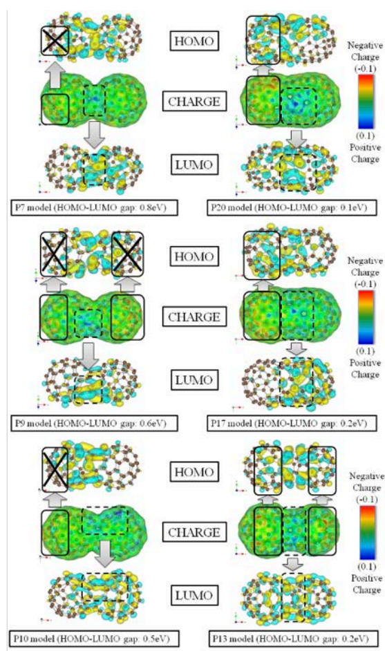
Figure 20. The correlation between the HOMO/LUMO wavefunction and effective charges for P7, P9, P10, P13, P17, and P20 isomers, where the red area of effective charges indicates negative charges (Maximum: -0.1) and the blue area indicates positive charges (Minimum: 0.1).
