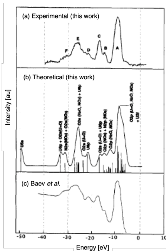
Figure 8. Experimental (a) and theoretical (b) XPS spectra of uranyl nitrate, \text{UO}_2(\text{NO}_3)_2 \cdot 2\text{H}_2\text{O} , along with the experimental spectrum (c) reported by Baev et al. [58].
