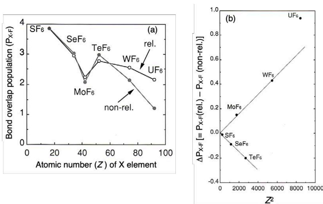
Figure 3. (a) Atomic-number ( Z ) dependence of bond overlap populations ( P_{X-F} ) for hexafluorides ( XF_6 ; X = S, Se, Mo, Te, W, U ), obtained using the non-relativistic DV-HFS and relativistic DV-DS methods, (b) Plot of the difference ( \Delta P_{X-F} ) in P_{X-F} between relativistic and non-relativistic calculations as a function of Z^2 .
