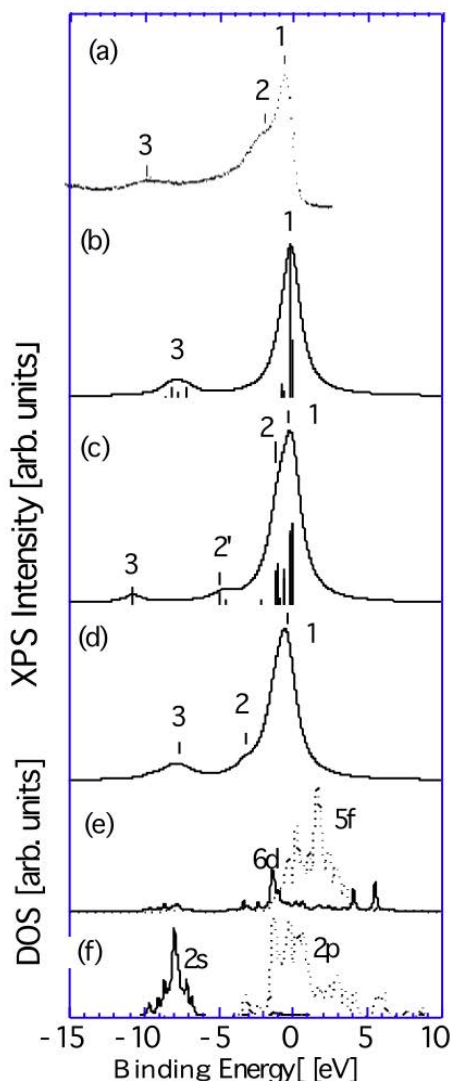
Figure 10. Theoretical and experimental valence x-ray photoelectron spectra for UC: (a) experiment [62] and theoretical spectra obtained using (b) \text{UC}_6 , (c) \text{CU}_6 , and (d) \text{CU}_6\text{C}_{18} cluster models, along with partial density-of-states (pDOS) for (e) the U5f (dashed line) and U6d (solid line) AOs and (f) the C2s (solid line) and C2p (dashed line) AOs.
