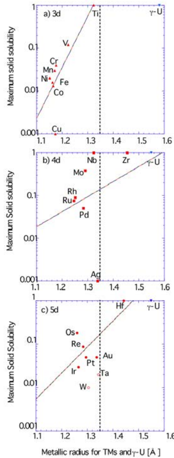
Figure 13. The correlation between the metallic radius of TMs and the maximum solid solubility (MSS) for \gamma -U alloyed with (a) 3d TMs, (b) 4d TMs, and (c) 5d TMs [Ref. 25].
