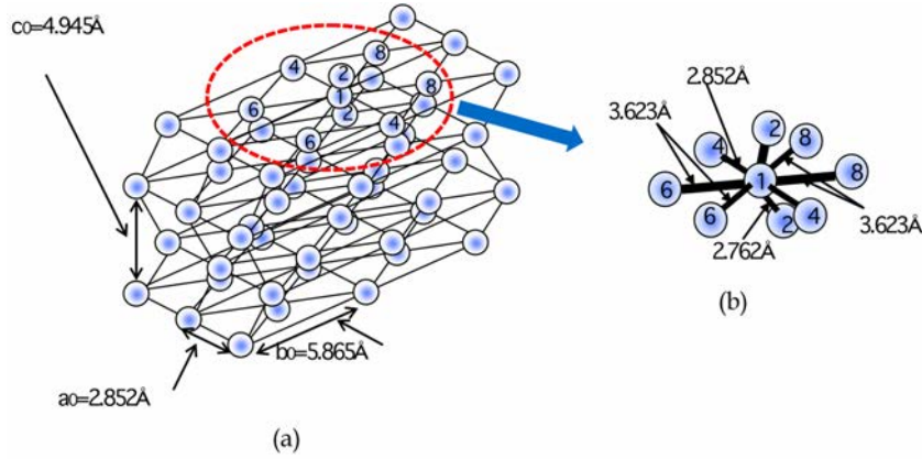
Figure 11. Schematic illustration of \alpha -U metal: (a) the orthorhombic structure of \alpha -U metal and (b) a U_9 cluster model used as the minimum unit of \alpha -U crystal structure [23].
