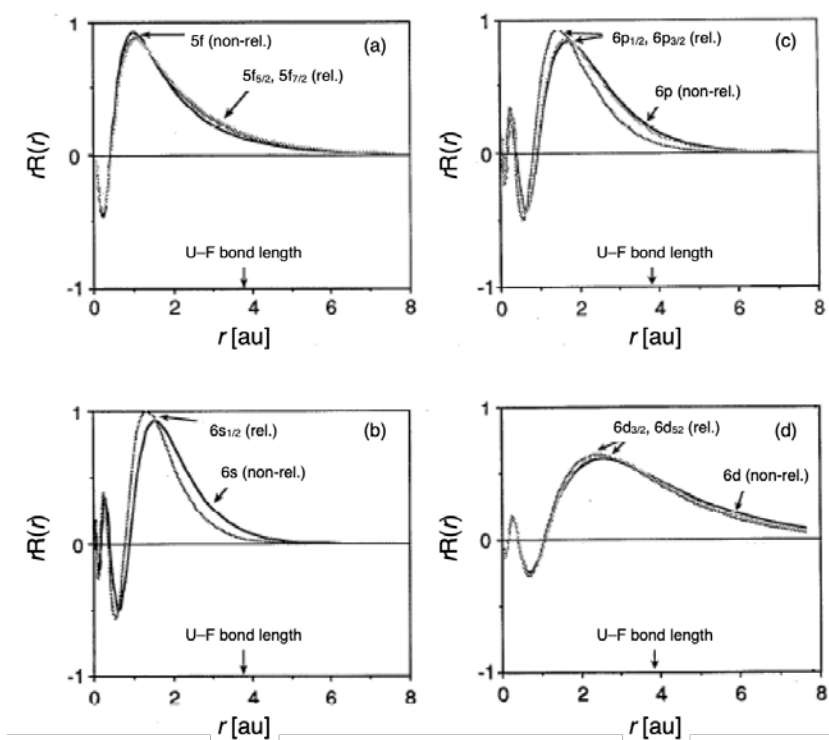
Figure 2. Comparison between non-relativistic and relativistic radial wave functions, [rR(r)] , of the valence AOs for uranium atom: (a) U5f, (b) U6s, (c) U6p, and (d) U6d. (FIG. 3 of Ref. 13 was partially modified.)
