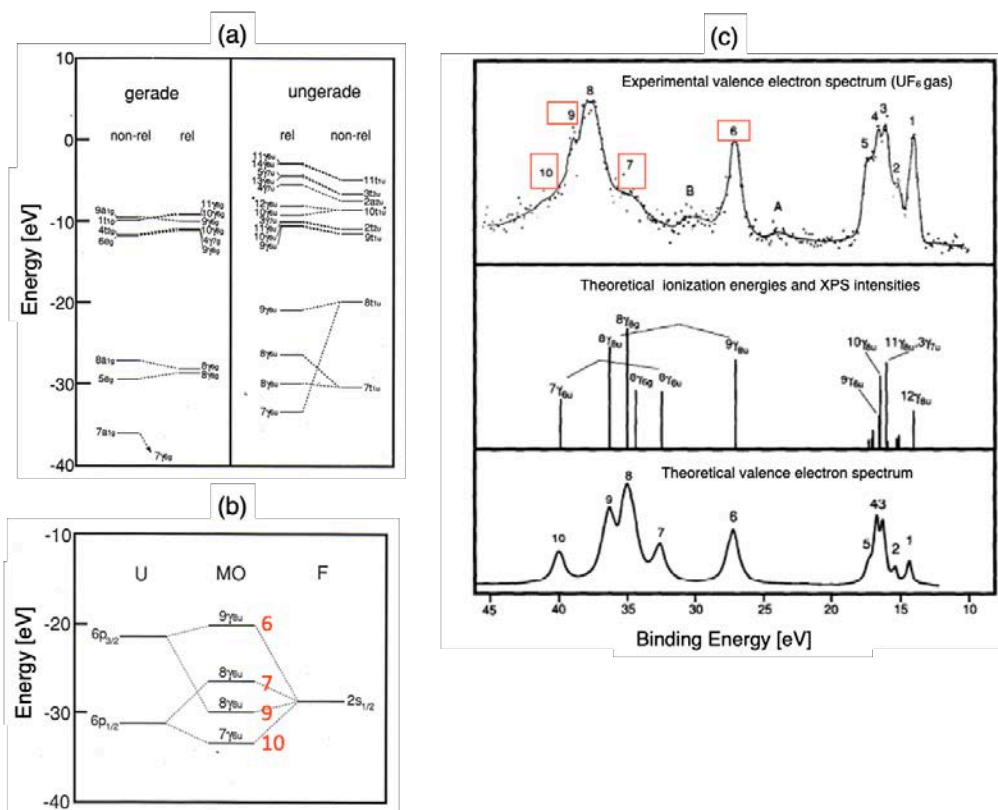
Figure 4. (a) Comparison of one-electron energies in the ground-state levels obtained for the nonrelativistic method with those for the relativistic one, (b) Schematic energy diagram representing the correlation among the lower valence MOs, U and F AOs, (c) Valence electron spectrum of \text{UF}_6 in a binding energy range of 0–50 eV: experimental valence photoelectron spectrum of gaseous \text{UF}_6 [38] (top); theoretical ionization energies and XPS intensities (the height of vertical line is proportional to the intensity) (middle); theoretical valence electron spectrum (bottom).
