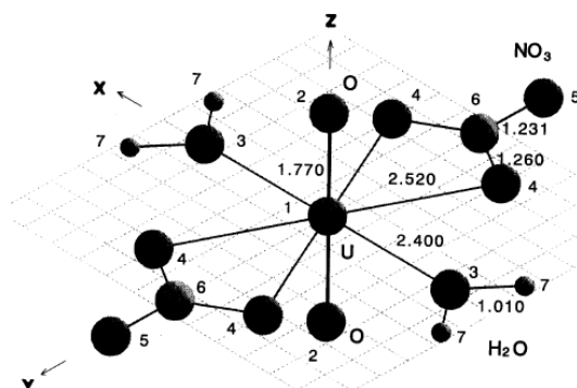
Figure 7. Schematic illustration of the structure of uranyl nitrate [58, 59]. Interatomic distances are shown in Ångströms.
