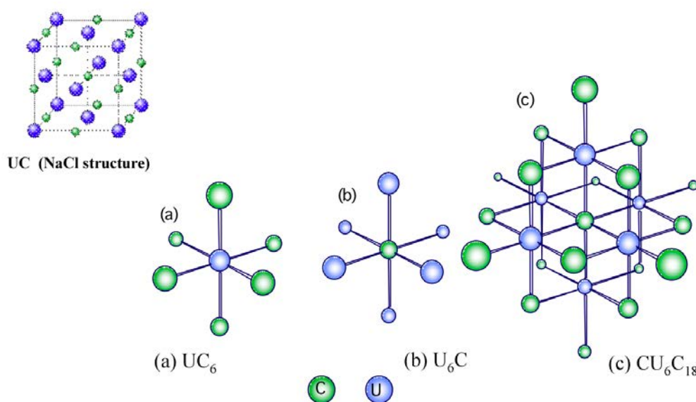
Figure 9. Schematic illustration of cluster models for UC with a NaCl-type crystal structure: (a) UC_6 , (b) CU_6 , and (c) CU_6C_{18} [Ref. 22].
