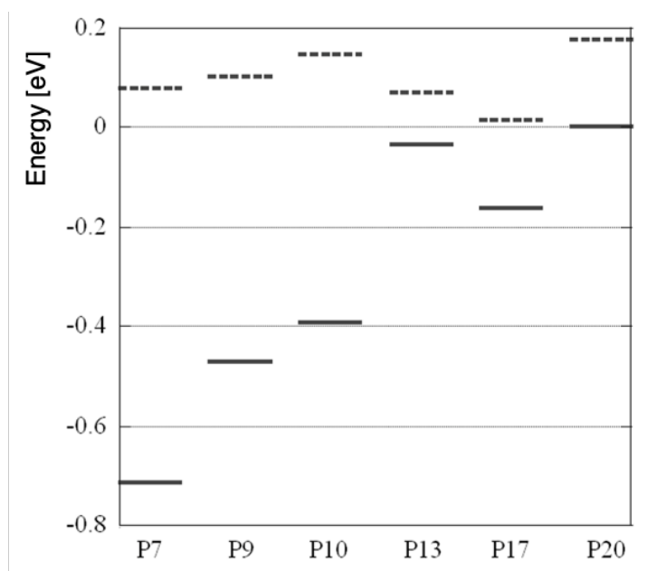
Figure 21. The energy level of the HOMO (solid line) and LUMO (dashed line) for P7, P9, P10, P13, P17, and P20 isomers.
