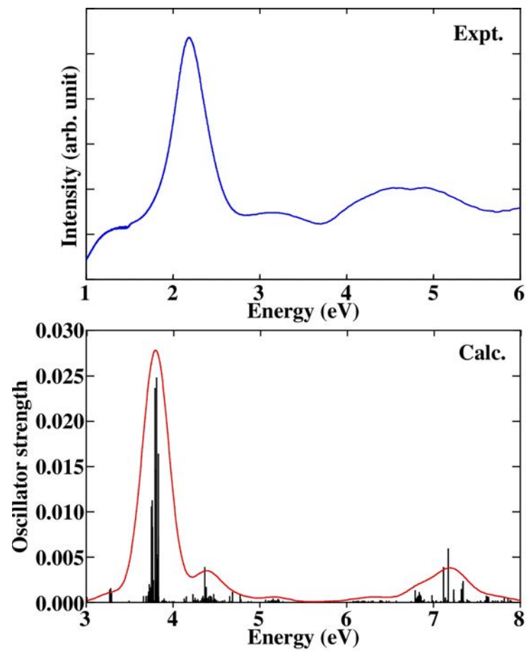
Figure 25. Comparison between the experimental (a) and theoretical (b) absorption spectra of FeFC (Prussian blue) [29].
