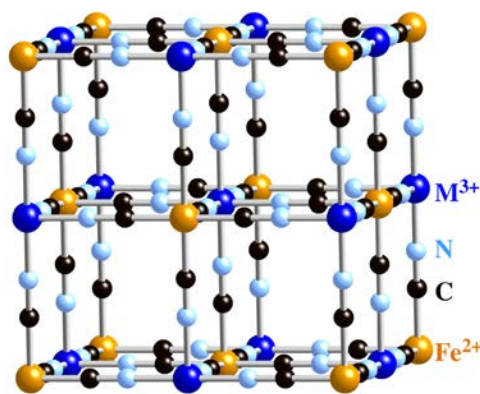
Figure 23. Schematic illustration of the crystal structure of M(III) ferrocyanides ( M=Fe, Co, Ni ), in which divalent iron ( Fe^{2+} ) and trivalent metal ( M^{3+} = Fe^{3+}, Co^{3+}, Ni^{3+} ) are bridged via the CN^- anion.
