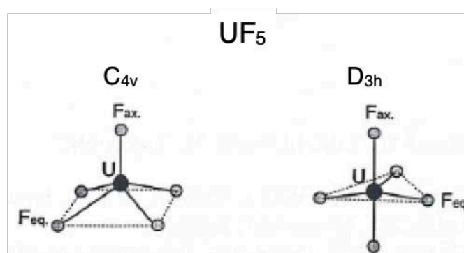
Figure 6. Schematic illustration of C 4v (U–F ax = 2.00 Å, U–F eq = 2.02 Å, F ax –U–F eq = 101°) and D 3h (U–F ax = 2.00 Å, U–F eq = 2.02 Å, F ax –U–F eq = 90°) geometries, which were experimentally and theoretically determined, respectively, for UF 5 molecule
