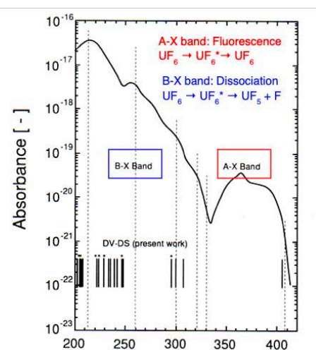
Figure 5. Comparison of excitation energies corresponding to F2p–U5f charge-transfer transitions between the present work and the experimental UV absorption spectrum of \text{UF}_6 [42].
