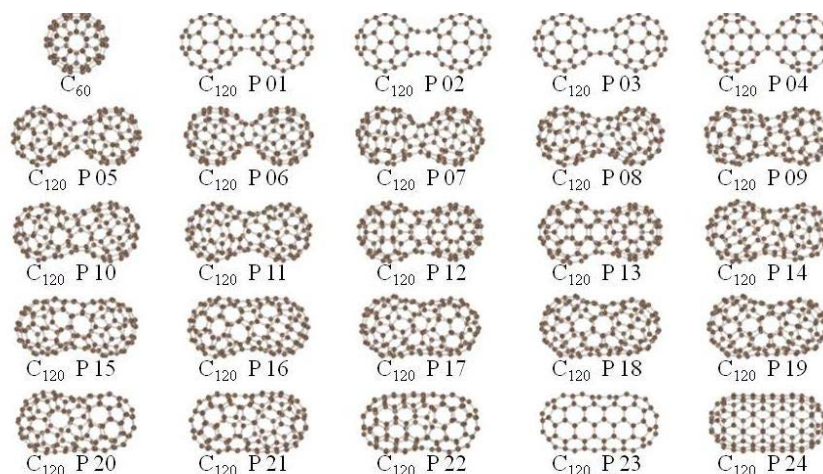
Figure 18. Schematic illustration of the stable C_{120} isomers derived from the general Stone-Wales rearrangement. Where, n -th C_{120} isomer is denoted as P_n [28].
