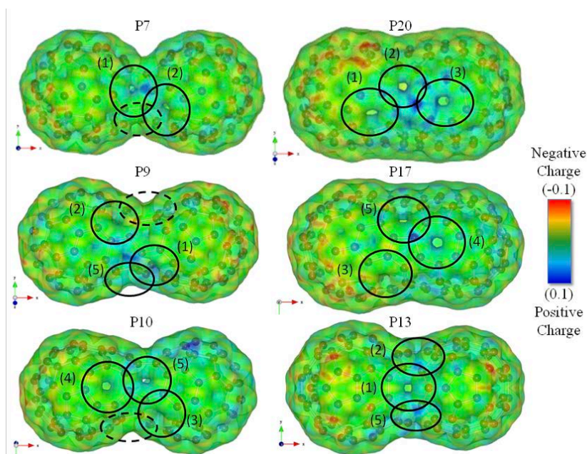
Figure 22. The effective charges and location of the 7-membered (solid circle) and 8-membered (dash circle) rings for P7, P9, P10, P13, P17, and P20 isomers, where the red area of effective charges has negative charges (Maximum: -0.1) and the blue one has positive charges (Minimum: 0.1).
