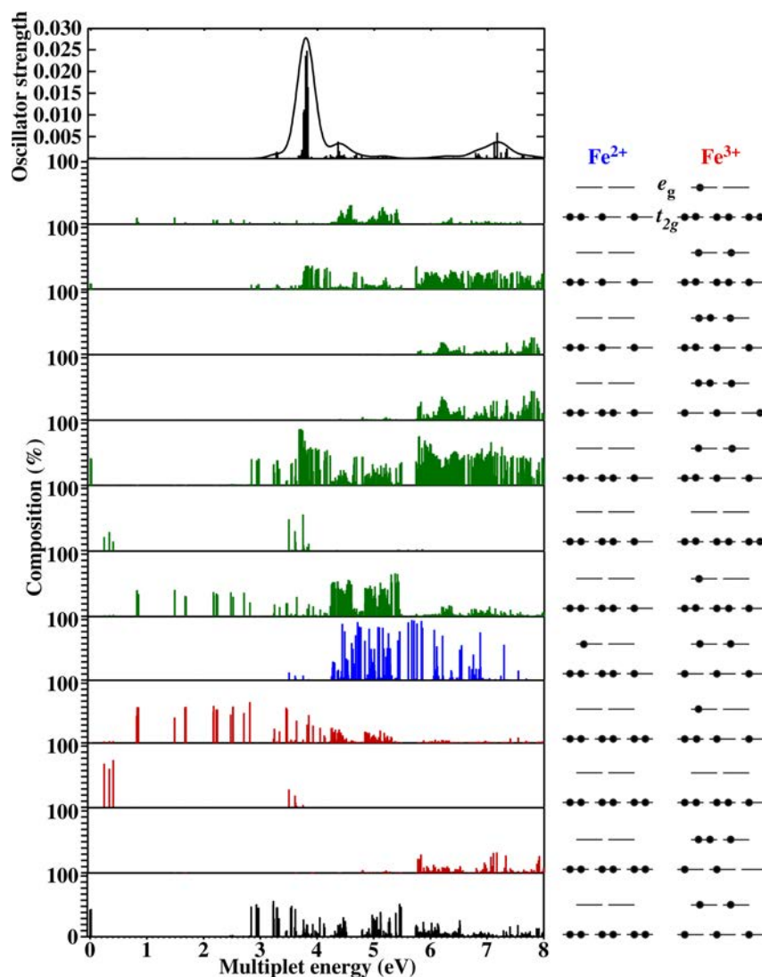
Figure 26. Configuration analysis of the many-electron wave functions for the 3d–3d intra-transitions and \text{Fe}^{2+} – \text{Fe}^{3+} CT transitions for FeFC. Corresponding electronic configurations are shown in right side.
