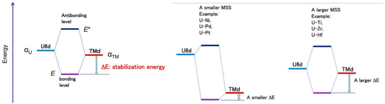
Figure 15. Schematic illustration of the TMd–U6d orbital interactions based on molecular orbital theory (left) and of the correlation between MSS and the stabilization energy ( \Delta E ) caused by their orbital interactions (right) [26].
