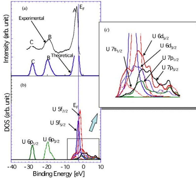
Figure 12. (a) Experimental [65] and theoretical spectra, (b) partial density-of-states (pDOS) of U valence AOs and (c) magnified pDOS in the vicinity of E_F [23].
