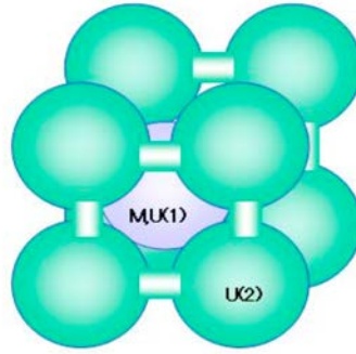
Figure 14. Schematic illustration of TM/ \gamma -U alloy cluster model: the central U atom (1) replaced with TM atom [24].
