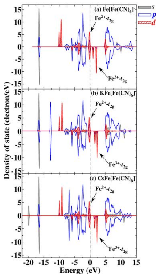
Figure 24. The DOS of FeFC calculated by using the three models: (a) \text{Fe}[\text{Fe}(\text{CN})_6]^- , (b) \text{KFe}[\text{Fe}(\text{CN})_6] , and (c) \text{CsFe}[\text{Fe}(\text{CN})_6] . The E_F is located at 0 eV along the energy axis. The occupied and unoccupied DOSs are located below and above the E_F , respectively. The positive and negative values of DOS indicate the up and down spin states, respectively. The partial DOS curves shown in gray, blue, and red denote s, p, and d-orbital, respectively.
