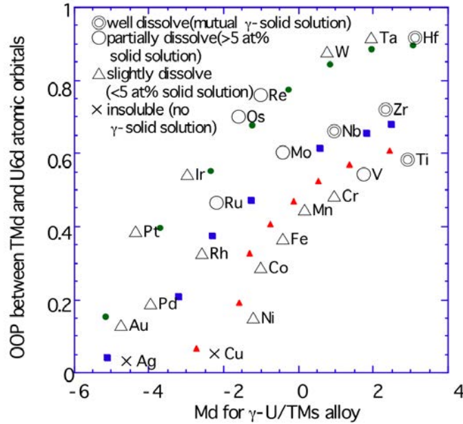
Figure 16. OOP vs. Md plot of \gamma -U/TM alloys [26].
